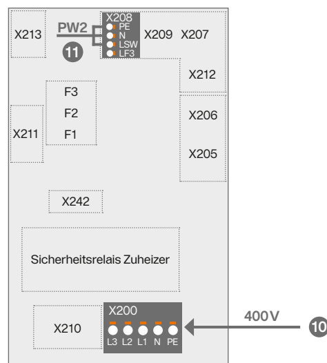
Inneneinheit Logatherm WLW186i TP70 XCU-SEH
